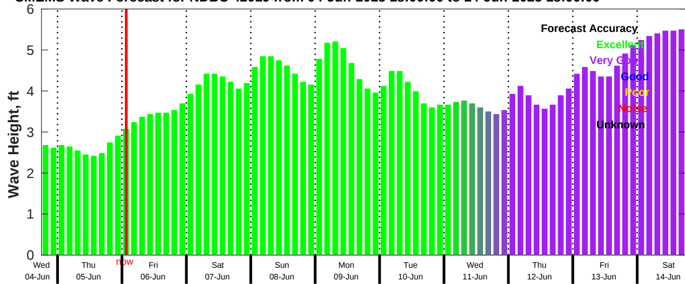
CMEMS Wave Forecast for NDBC 42019 from 04-Jun-2025 18:00:00 to 14-Jun-2025 18:00:00
