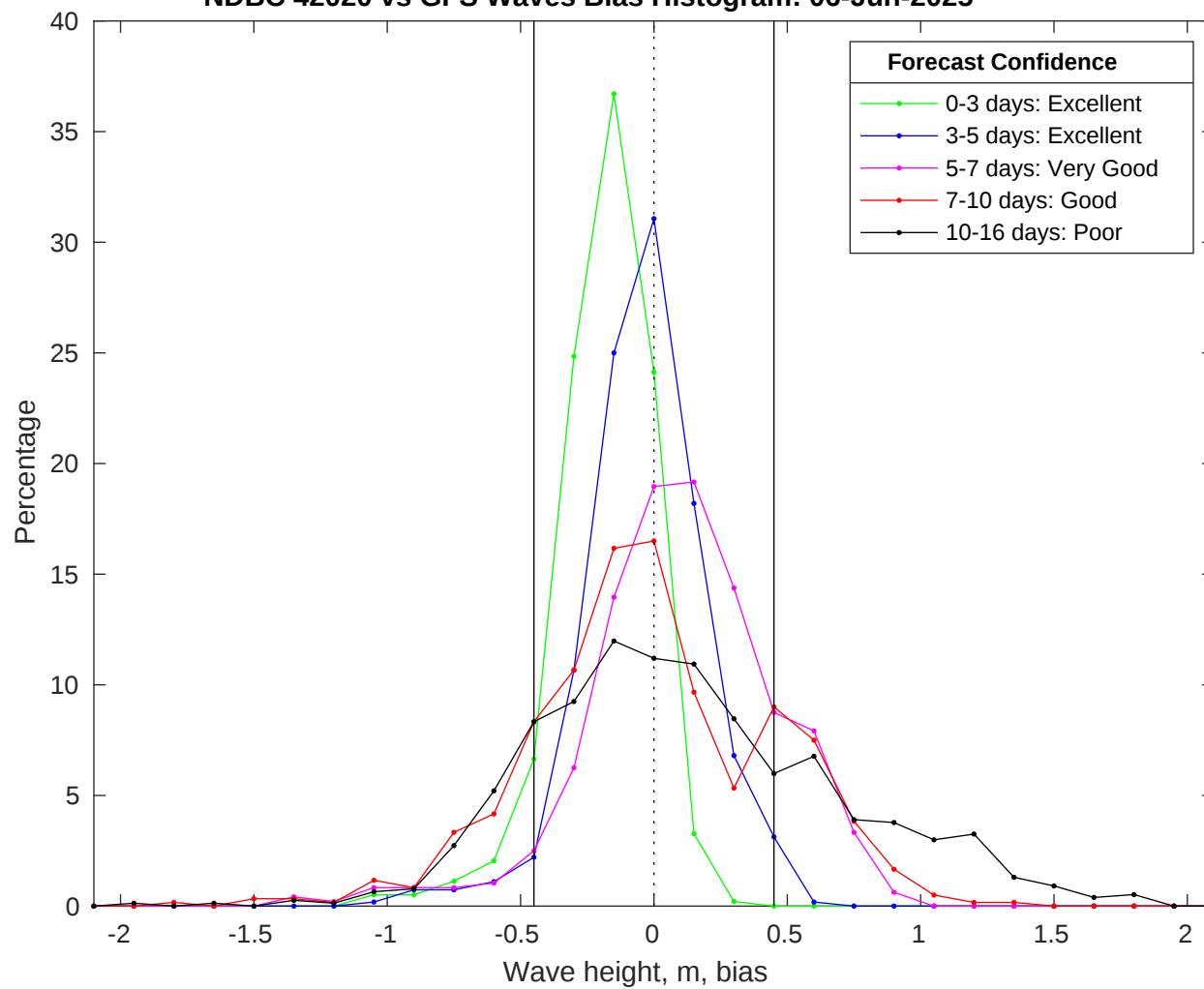
NDBC 42020 vs GFS Waves Bias Histogram: 06-Jun-2025
