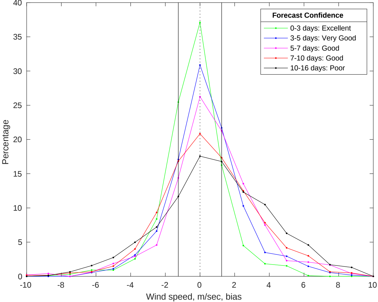
NDBC 42020 vs GFS Winds Bias Histogram: 06-Jun-2025
