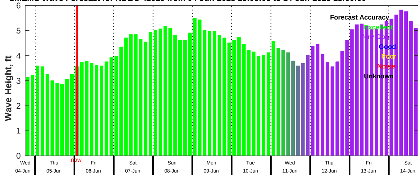
CMEMS Wave Forecast for NDBC 42020 from 04-Jun-2025 18:00:00 to 14-Jun-2025 18:00:00
