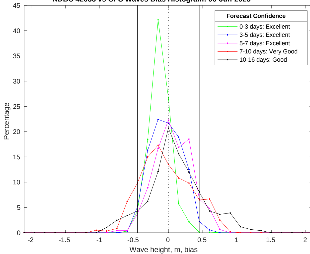
NDBC 42035 vs GFS Waves Bias Histogram: 06-Jun-2025
