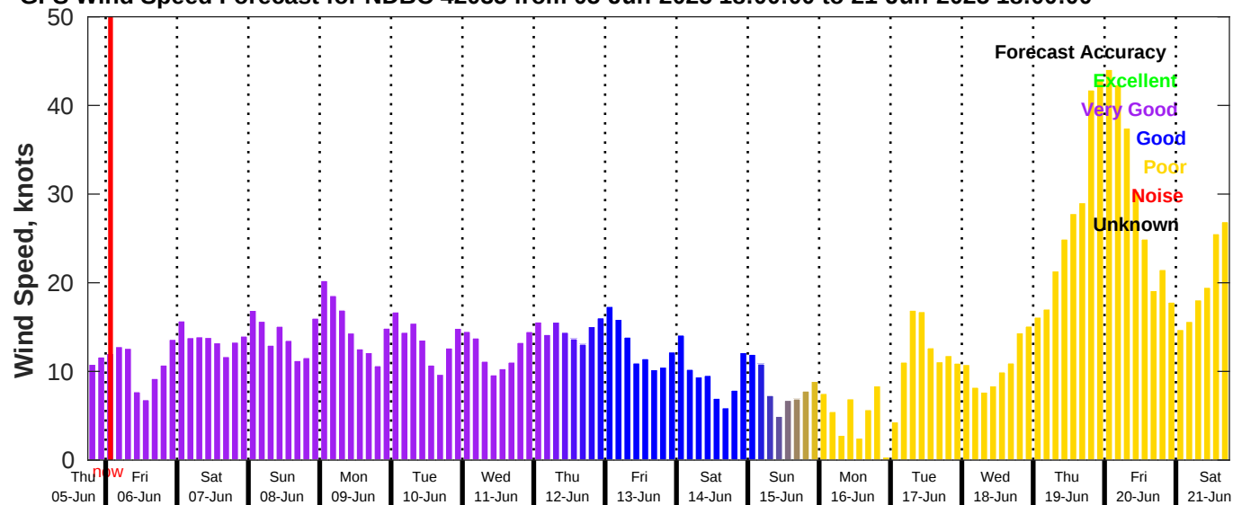
GFS Wind Speed Forecast for NDBC 42035 from 05-Jun-2025 18:00:00 to 21-Jun-2025 18:00:00
