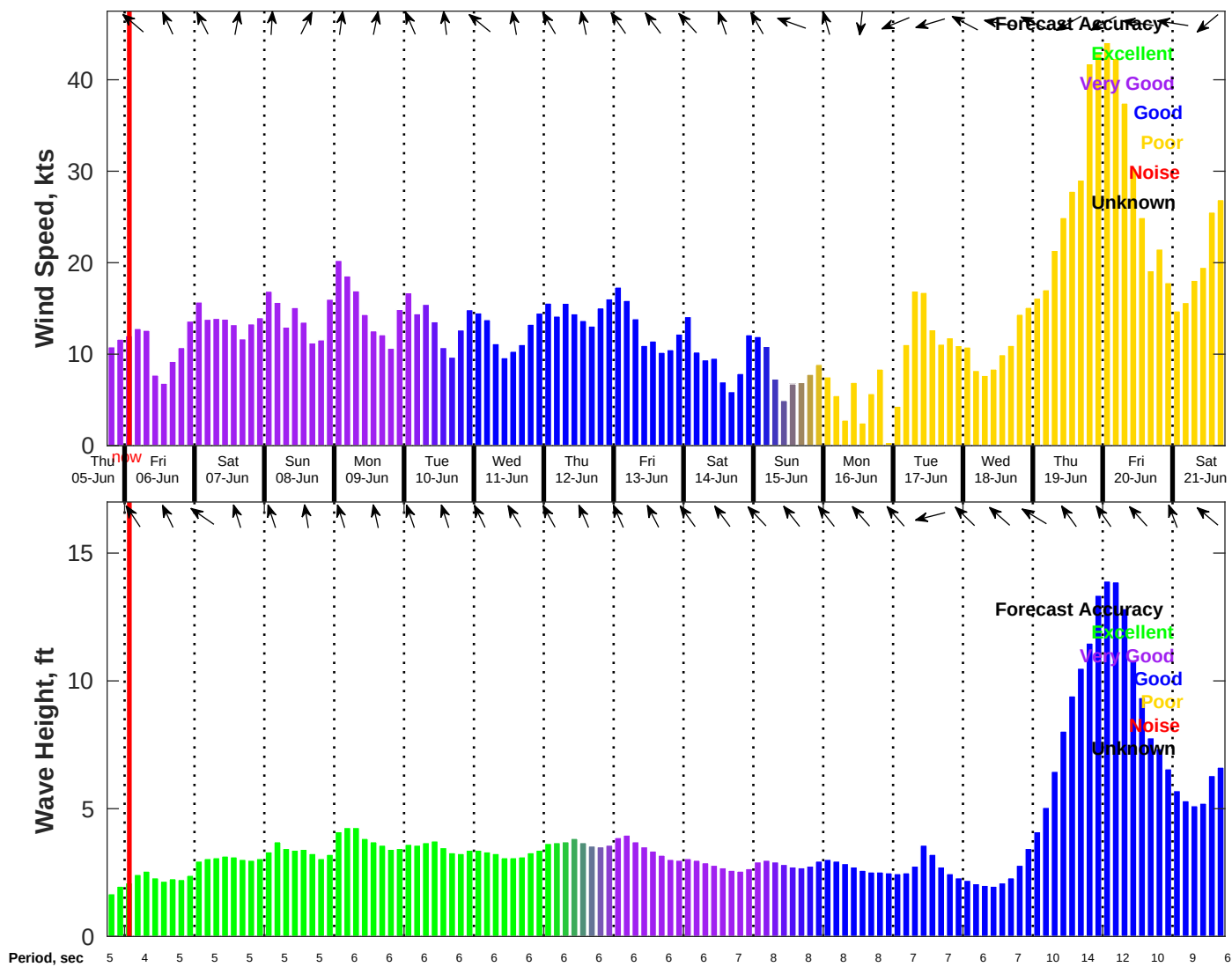
Wind & Wave Forecast for NDBC 42035 from 05-Jun-2025 18:00:00 to 21-Jun-2025 18:00:00
