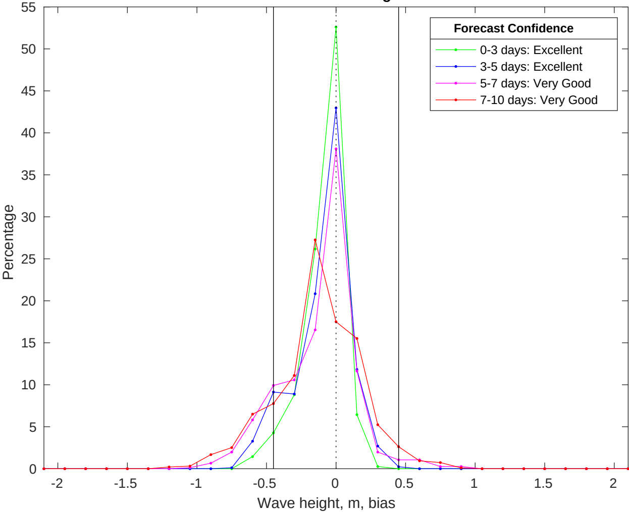
NDBC 42036 vs CMEMS Waves Bias Histogram: 06-Jun-2025
