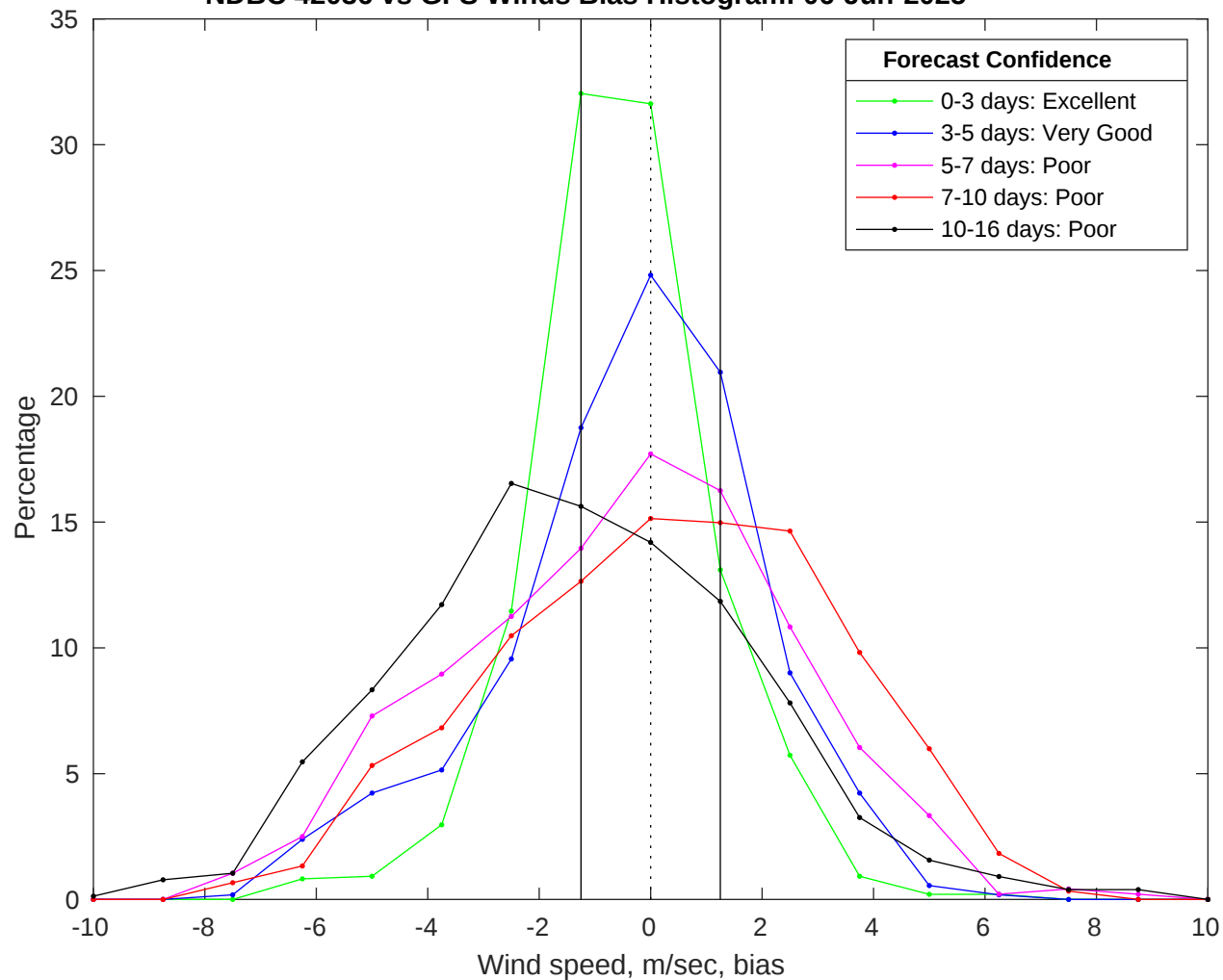
NDBC 42036 vs GFS Winds Bias Histogram: 06-Jun-2025
