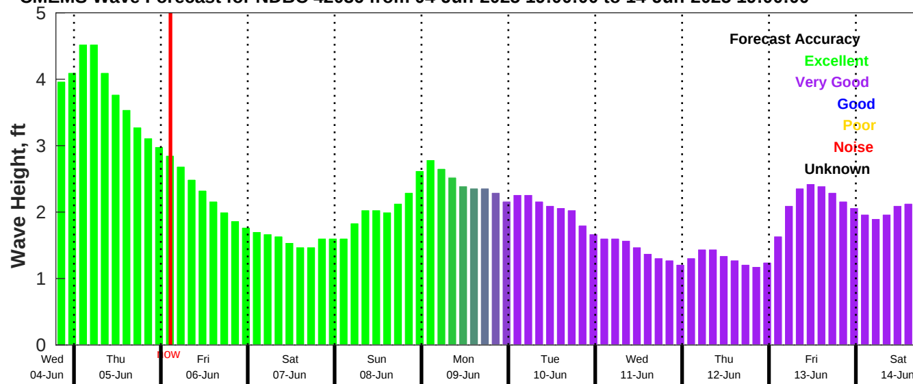
CMEMS Wave Forecast for NDBC 42036 from 04-Jun-2025 19:00:00 to 14-Jun-2025 19:00:00
