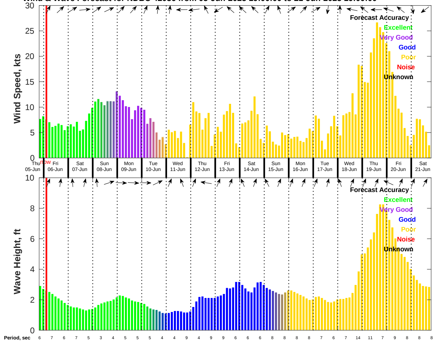
Wind & Wave Forecast for NDBC 42036 from 05-Jun-2025 19:00:00 to 21-Jun-2025 19:00:00
