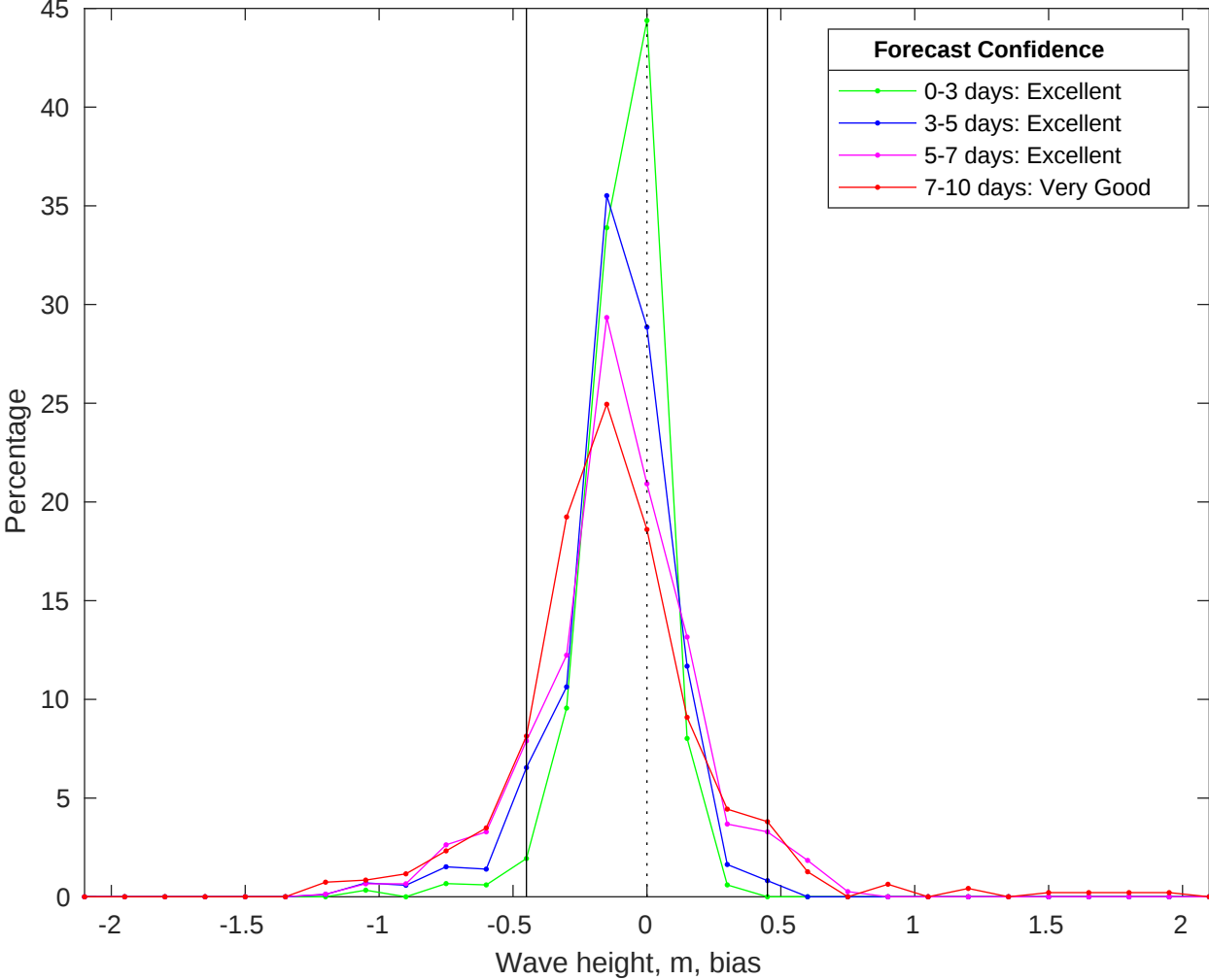
NDBC 42040 vs CMEMS Waves Bias Histogram: 06-Jun-2025
