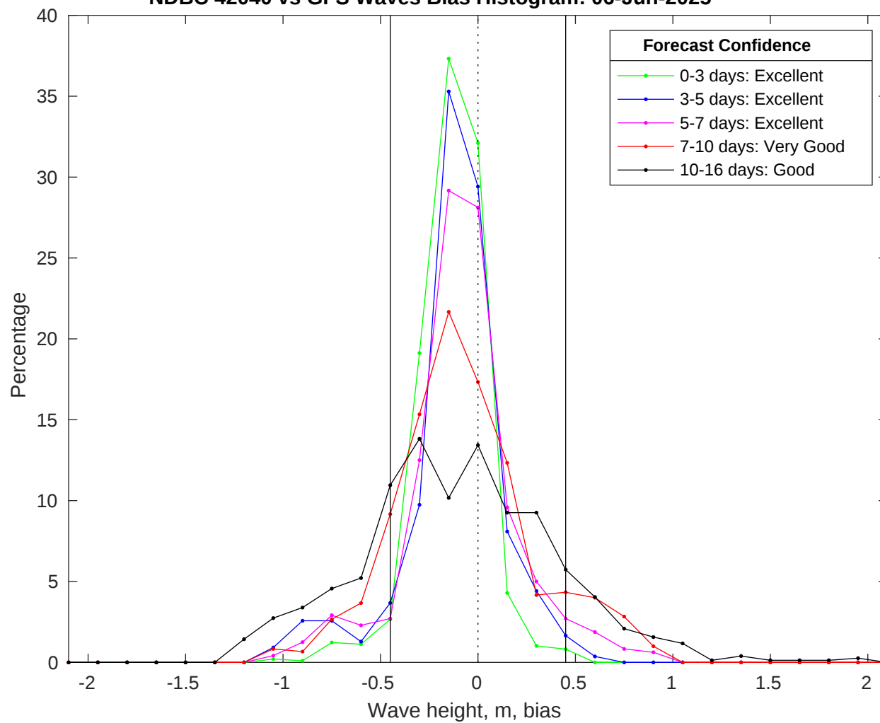
NDBC 42040 vs GFS Waves Bias Histogram: 06-Jun-2025
