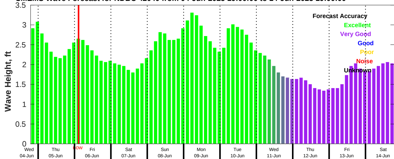
CMEMS Wave Forecast for NDBC 42040 from 04-Jun-2025 19:00:00 to 14-Jun-2025 19:00:00
