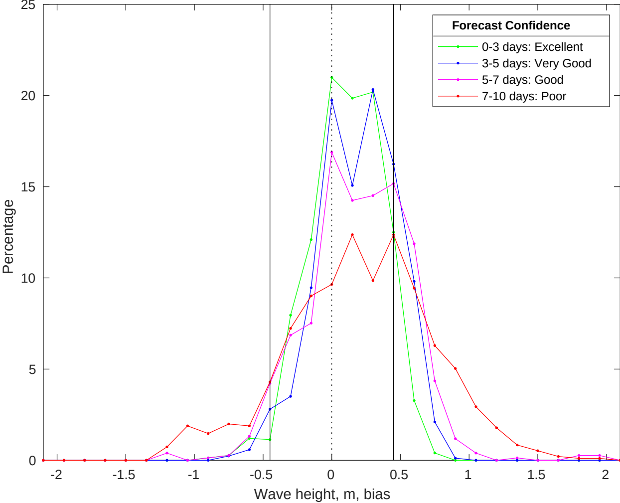
NDBC 46011 vs CMEMS Waves Bias Histogram: 06-Jun-2025
