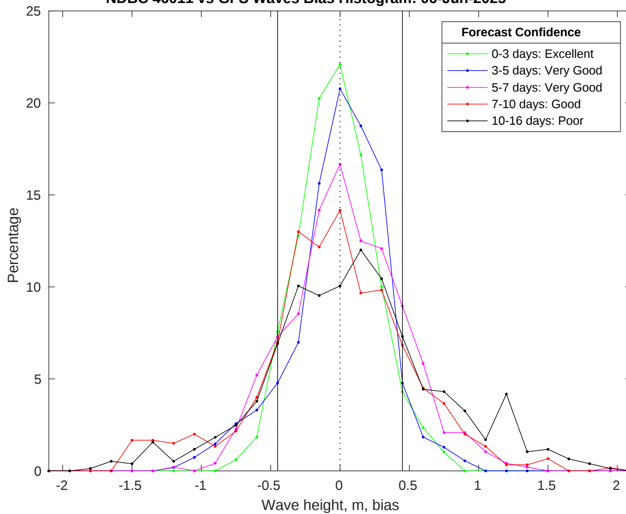
NDBC 46011 vs GFS Waves Bias Histogram: 06-Jun-2025
