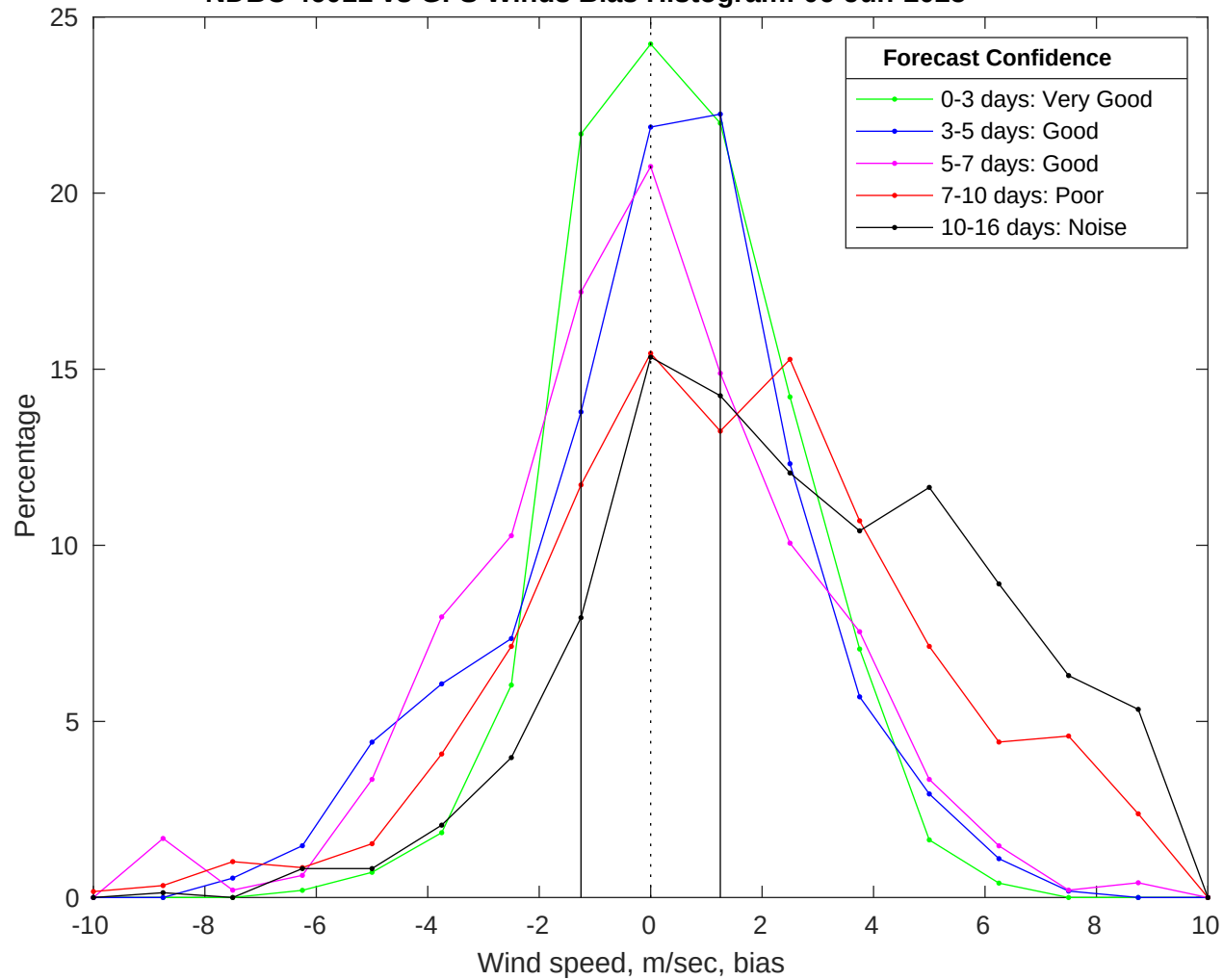
NDBC 46011 vs GFS Winds Bias Histogram: 06-Jun-2025
