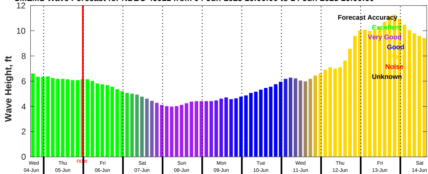
CMEMS Wave Forecast for NDBC 46011 from 04-Jun-2025 16:00:00 to 14-Jun-2025 16:00:00
