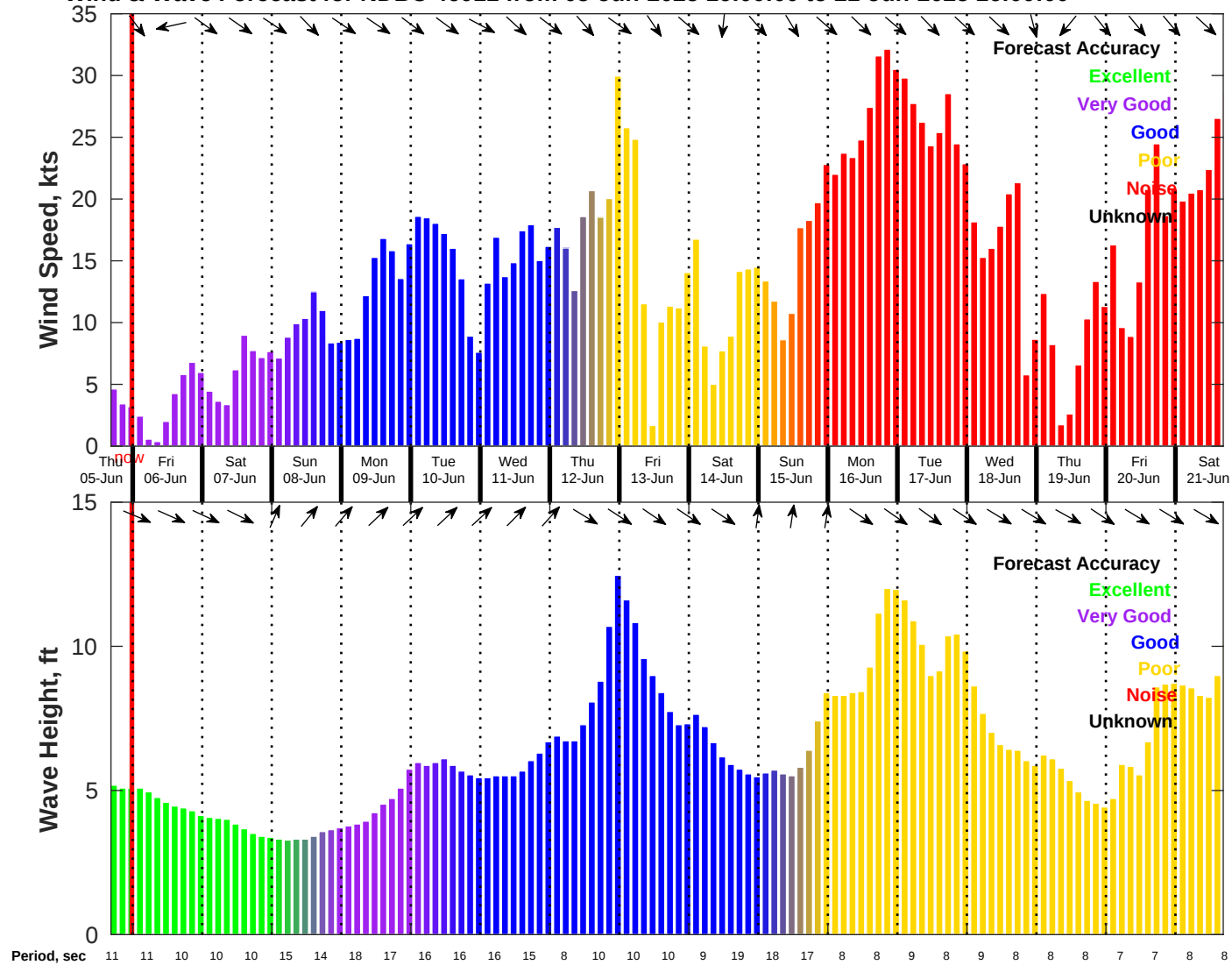
Wind & Wave Forecast for NDBC 46011 from 05-Jun-2025 16:00:00 to 21-Jun-2025 16:00:00
