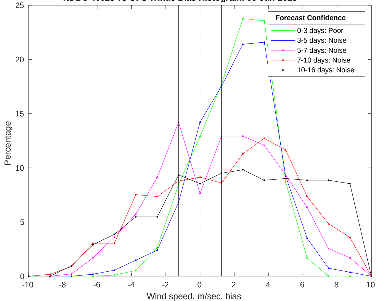
NDBC 46028 vs GFS Winds Bias Histogram: 06-Jun-2025
