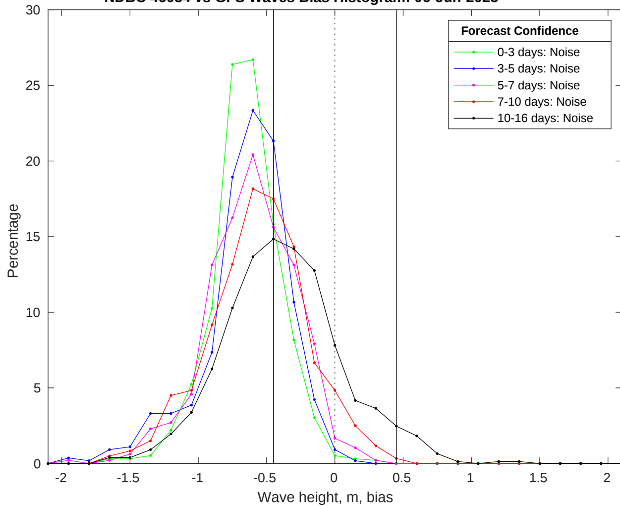
NDBC 46054 vs GFS Waves Bias Histogram: 06-Jun-2025
