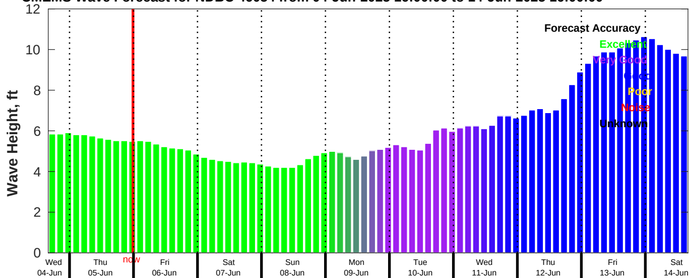
CMEMS Wave Forecast for NDBC 46054 from 04-Jun-2025 16:00:00 to 14-Jun-2025 16:00:00
