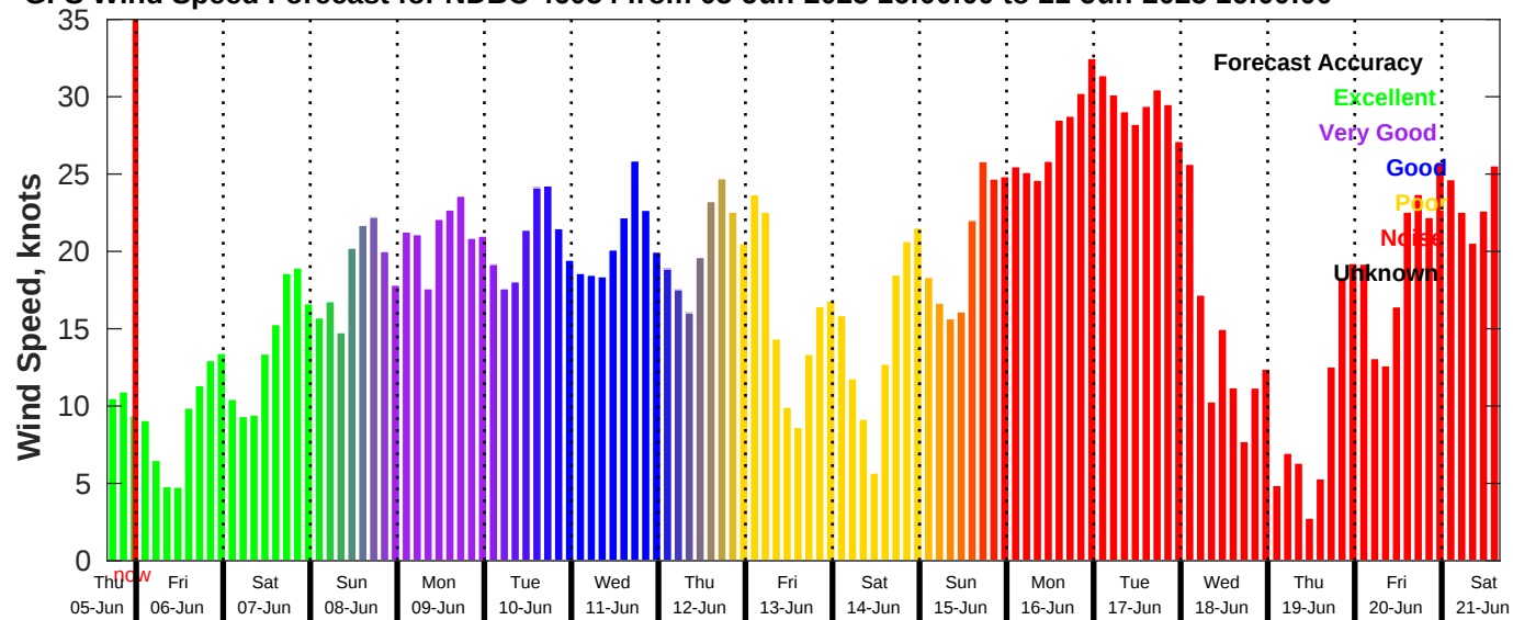
GFS Wind Speed Forecast for NDBC 46054 from 05-Jun-2025 16:00:00 to 21-Jun-2025 16:00:00
