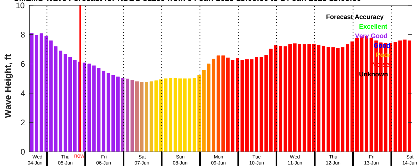
CMEMS Wave Forecast for NDBC 51209 from 04-Jun-2025 13:00:00 to 14-Jun-2025 13:00:00
