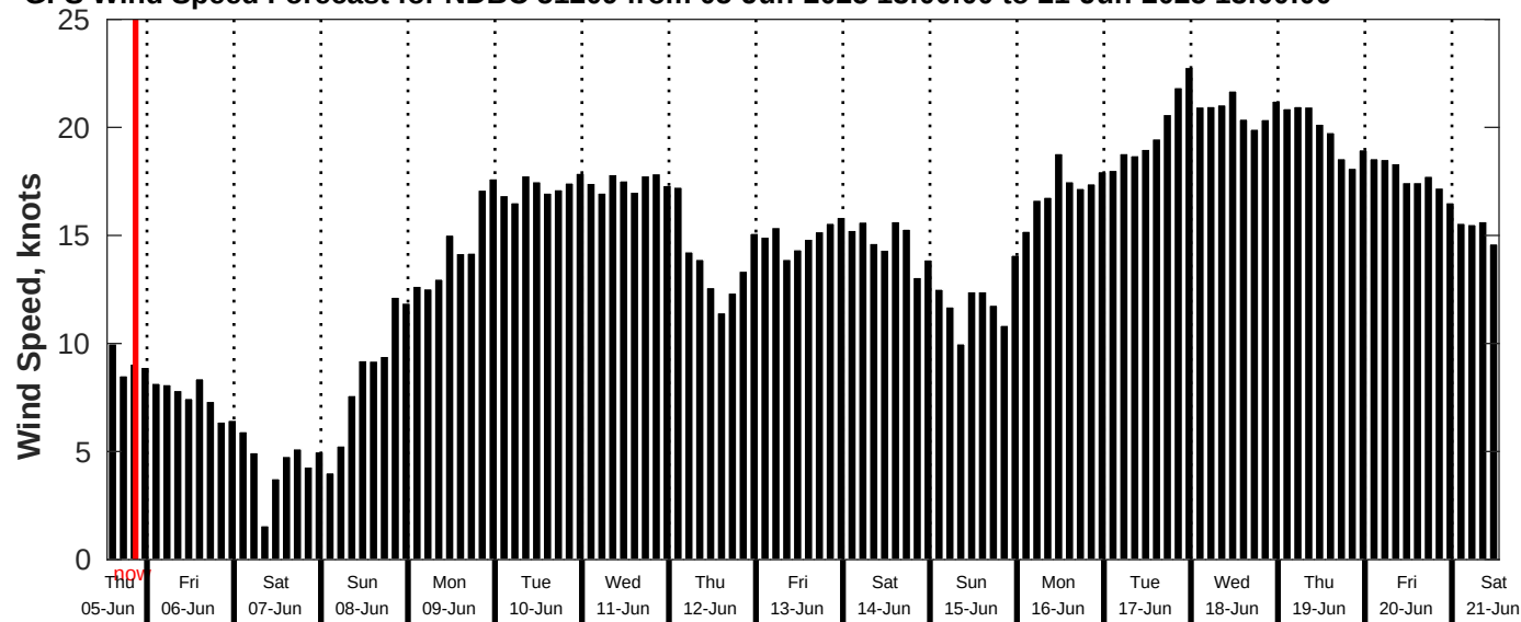
GFS Wind Speed Forecast for NDBC 51209 from 05-Jun-2025 13:00:00 to 21-Jun-2025 13:00:00
