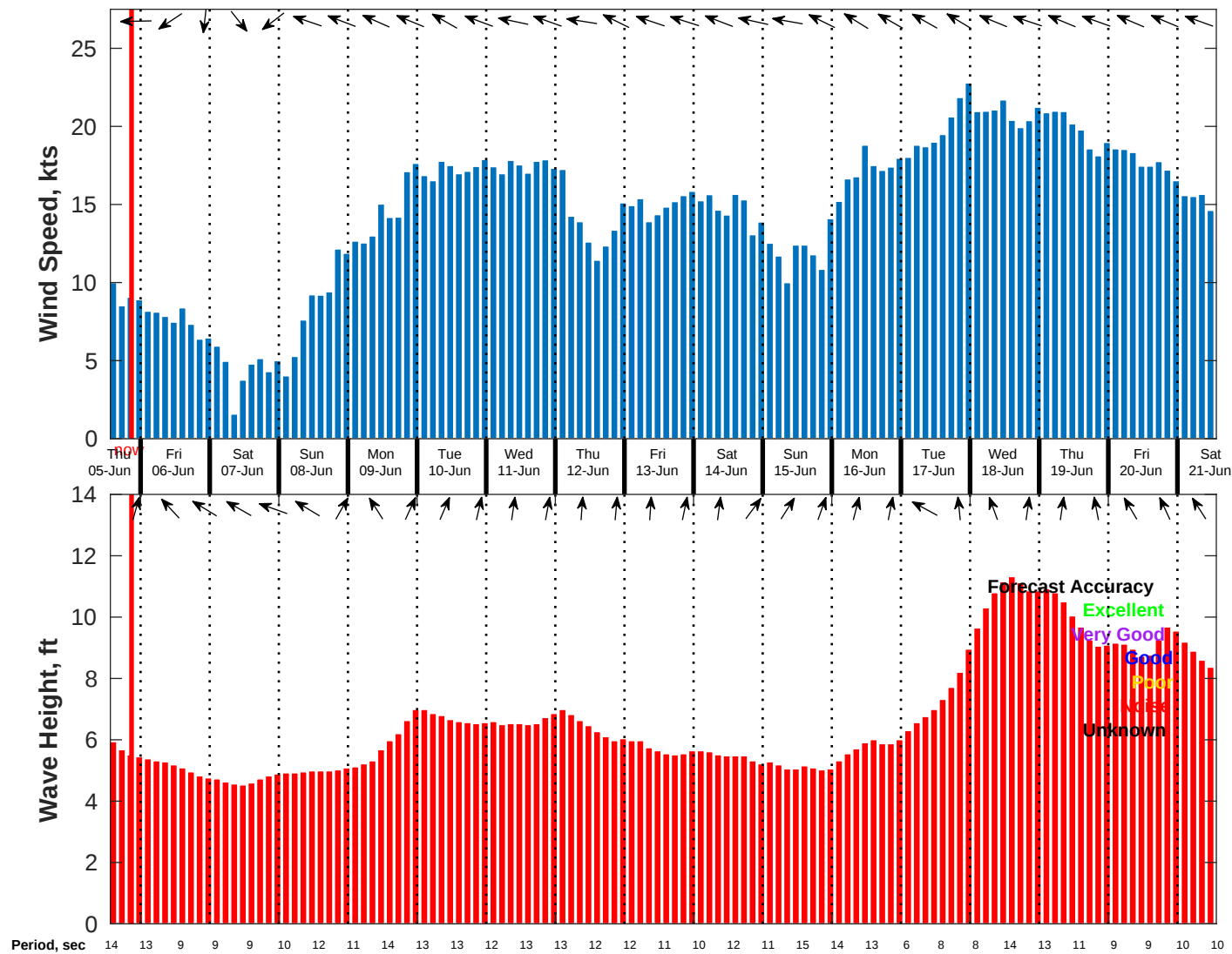
Wind & Wave Forecast for NDBC 51209 from 05-Jun-2025 13:00:00 to 21-Jun-2025 13:00:00
