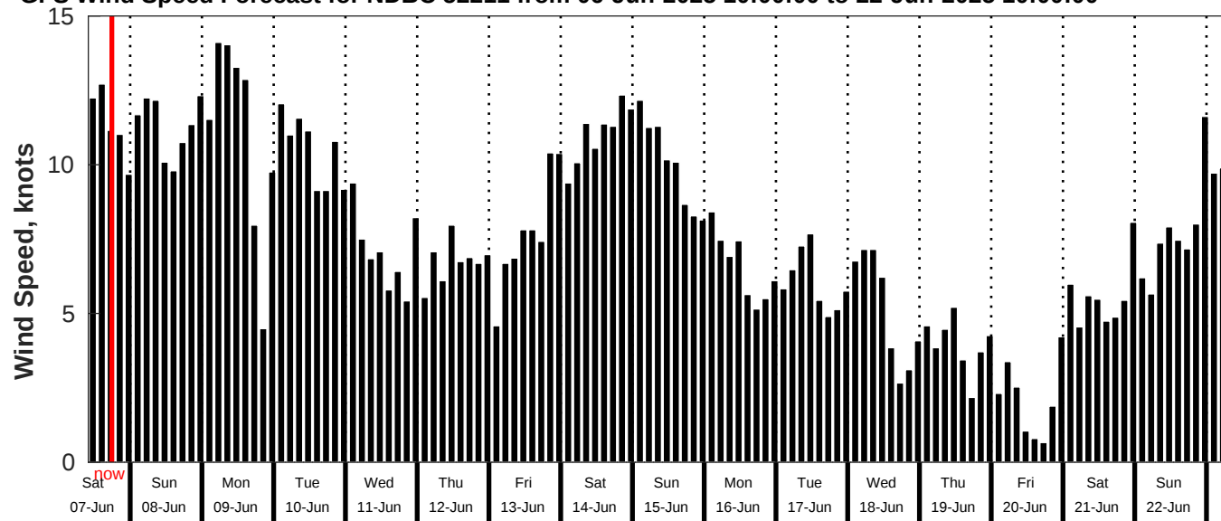
GFS Wind Speed Forecast for NDBC 52211 from 06-Jun-2025 10:00:00 to 22-Jun-2025 10:00:00
