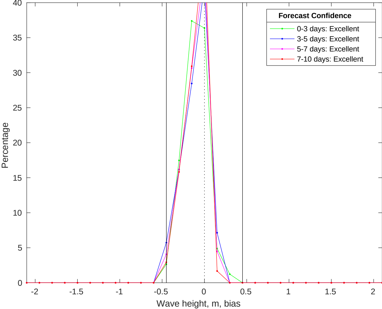
NDBC 52212 vs CMEMS Waves Bias Histogram: 06-Jun-2025
