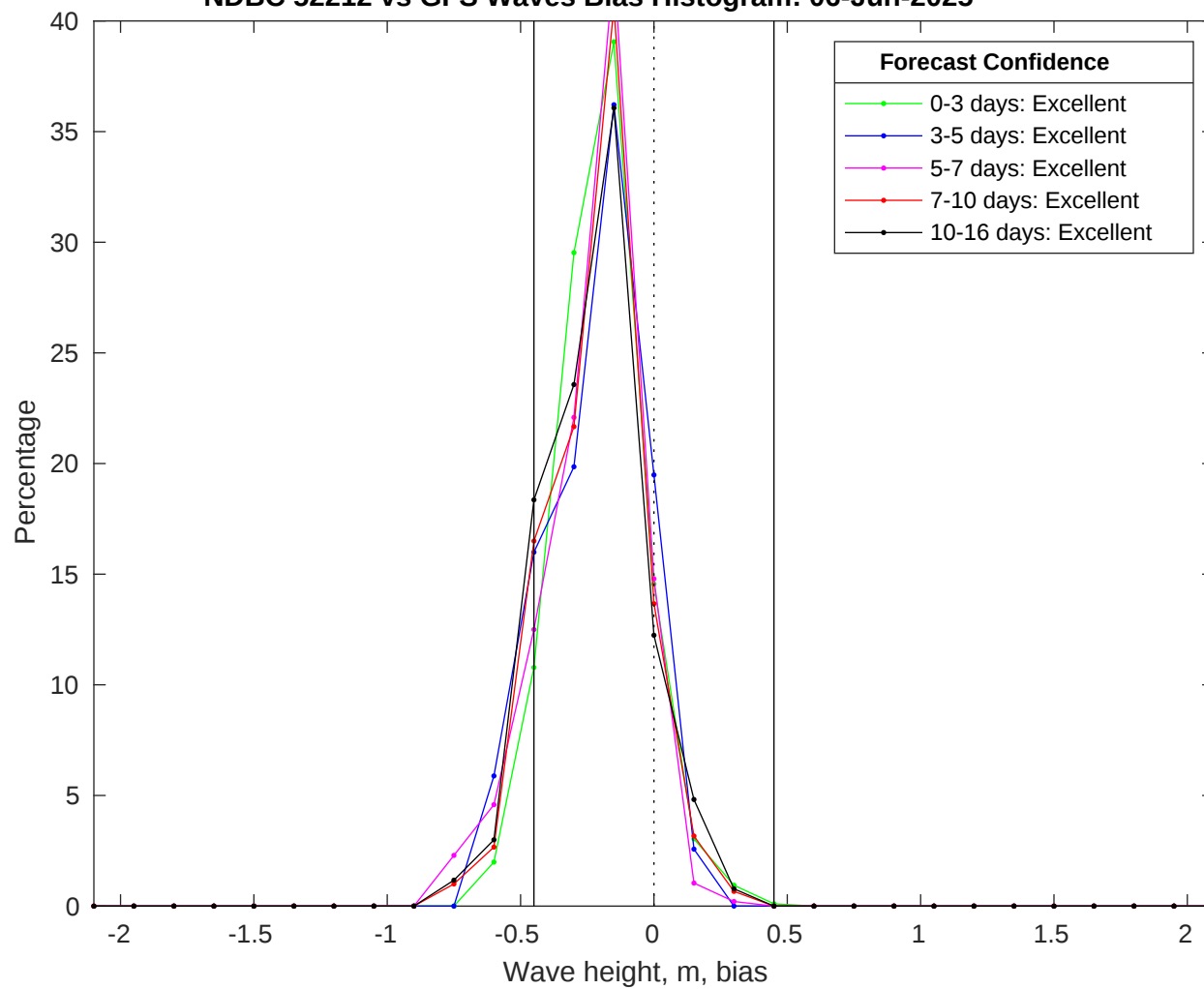
NDBC 52212 vs GFS Waves Bias Histogram: 06-Jun-2025
