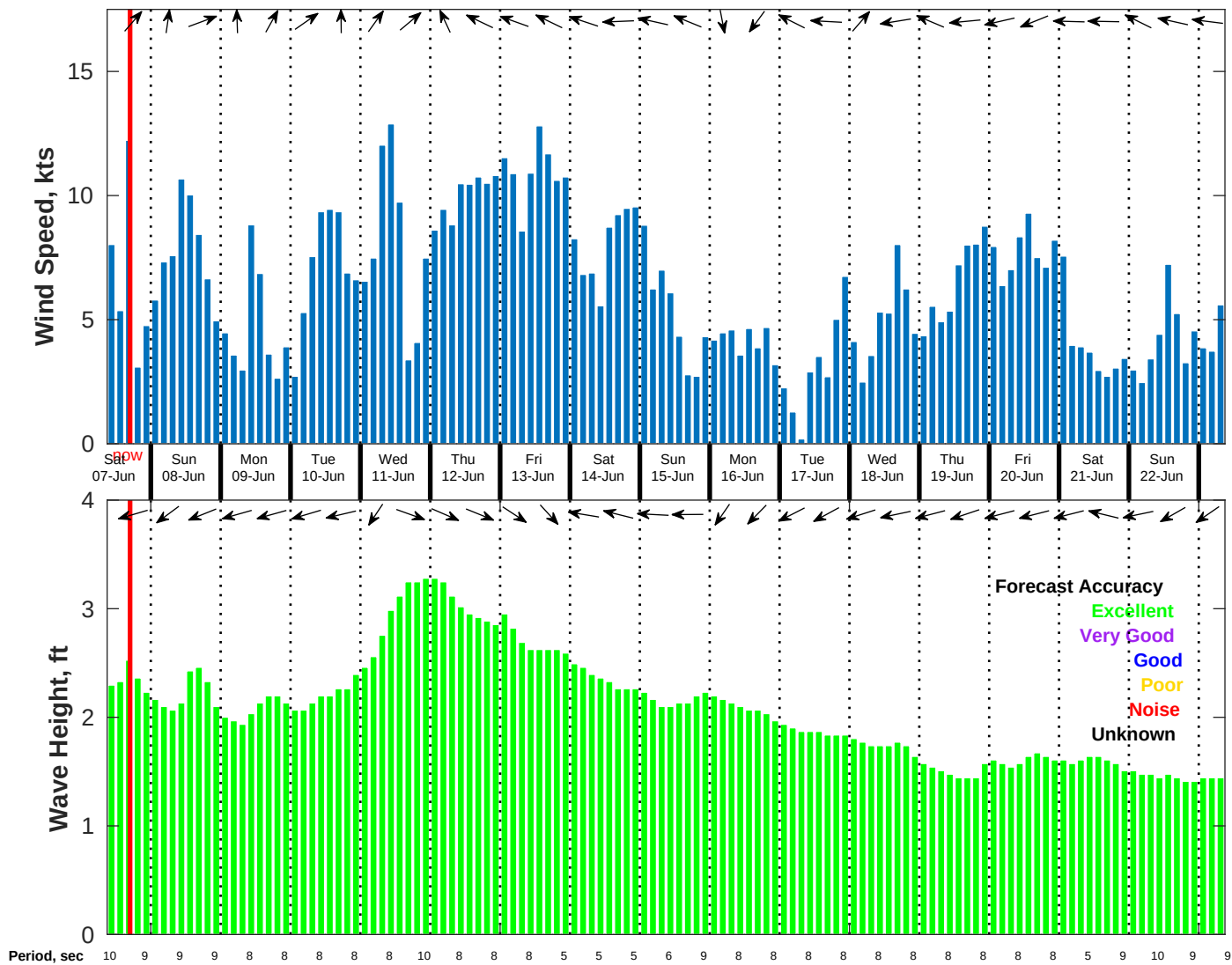
Wind & Wave Forecast for NDBC 52212 from 06-Jun-2025 09:00:00 to 22-Jun-2025 09:00:00
