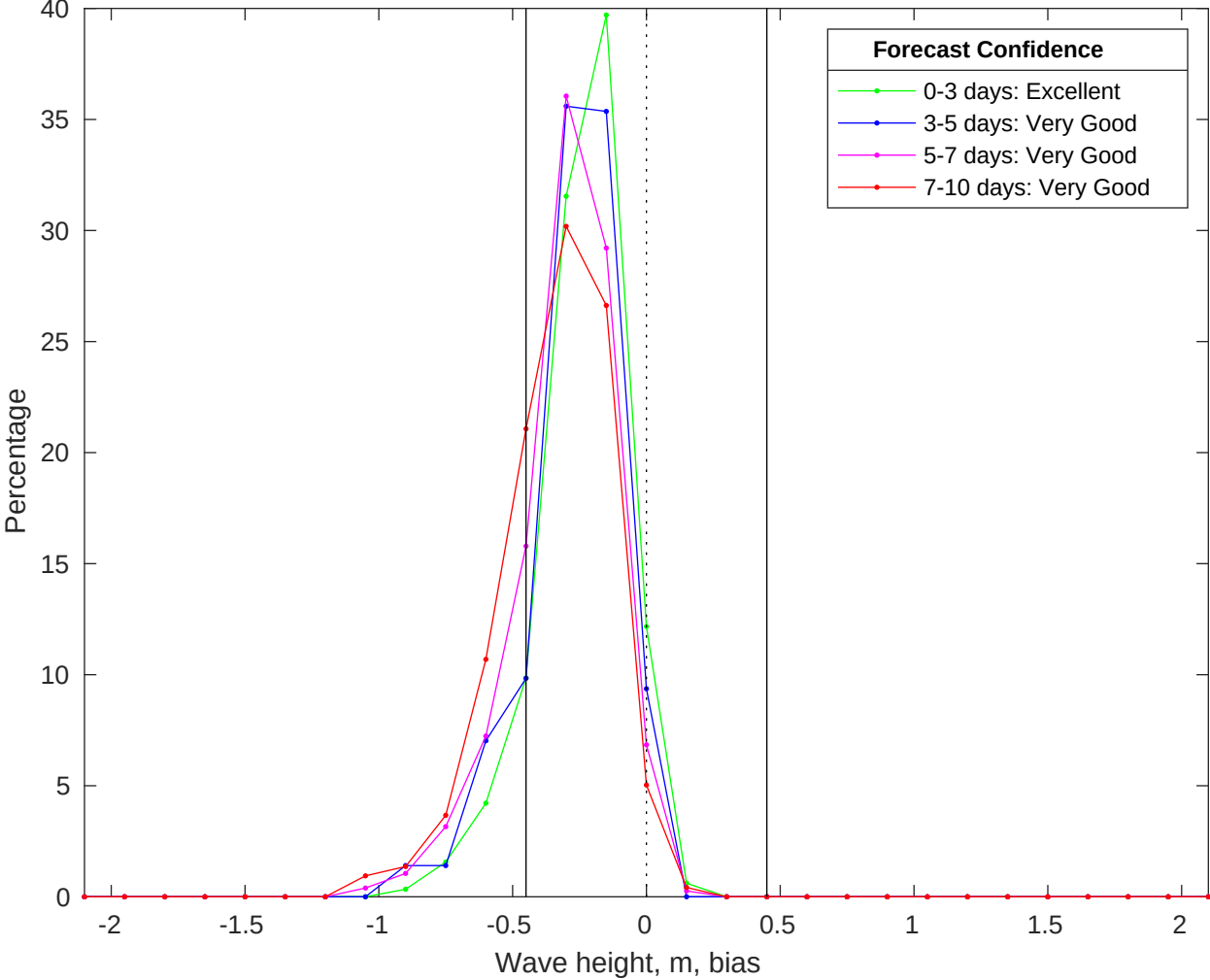
NDBC 52213 vs CMEMS Waves Bias Histogram: 06-Jun-2025
