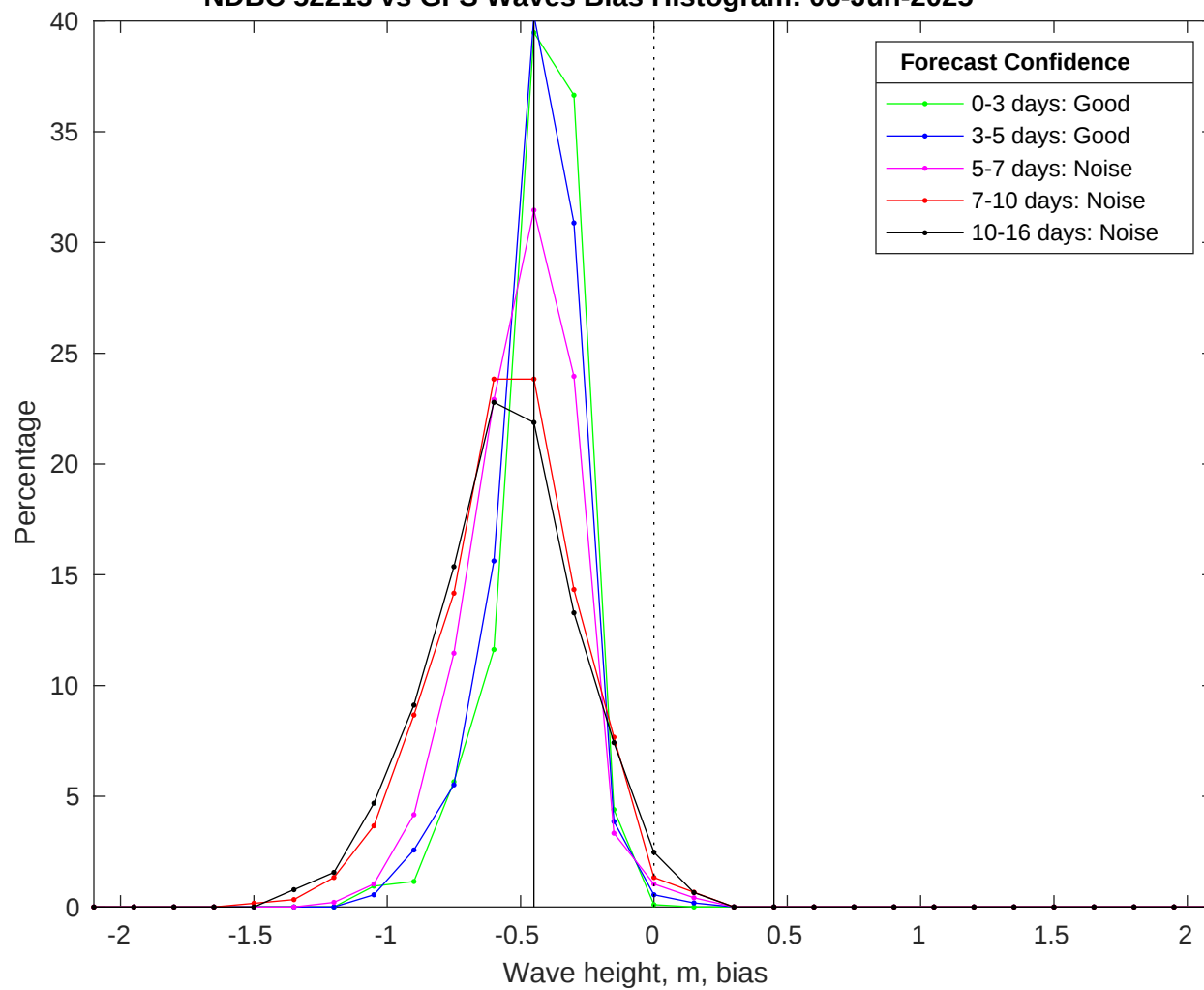
NDBC 52213 vs GFS Waves Bias Histogram: 06-Jun-2025
