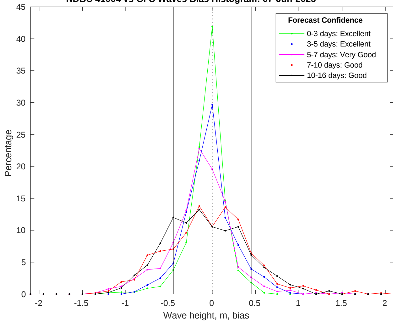
NDBC 41004 vs GFS Waves Bias Histogram: 07-Jun-2025
