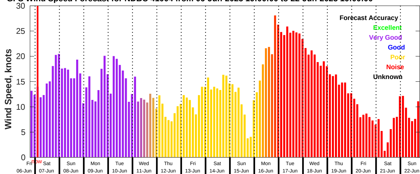
GFS Wind Speed Forecast for NDBC 41004 from 06-Jun-2025 19:00:00 to 22-Jun-2025 19:00:00
