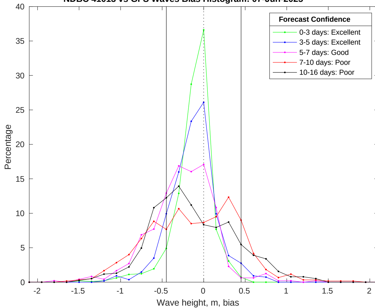
NDBC 41013 vs GFS Waves Bias Histogram: 07-Jun-2025
