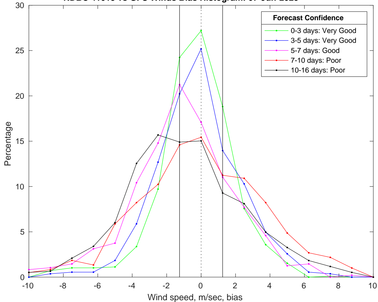
NDBC 41013 vs GFS Winds Bias Histogram: 07-Jun-2025
