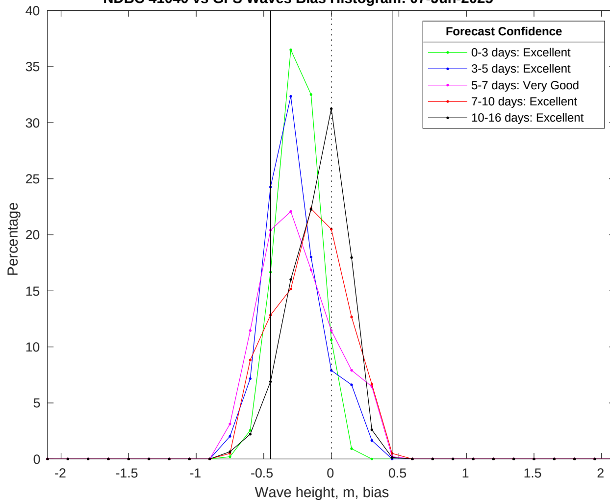
NDBC 41040 vs GFS Waves Bias Histogram: 07-Jun-2025
