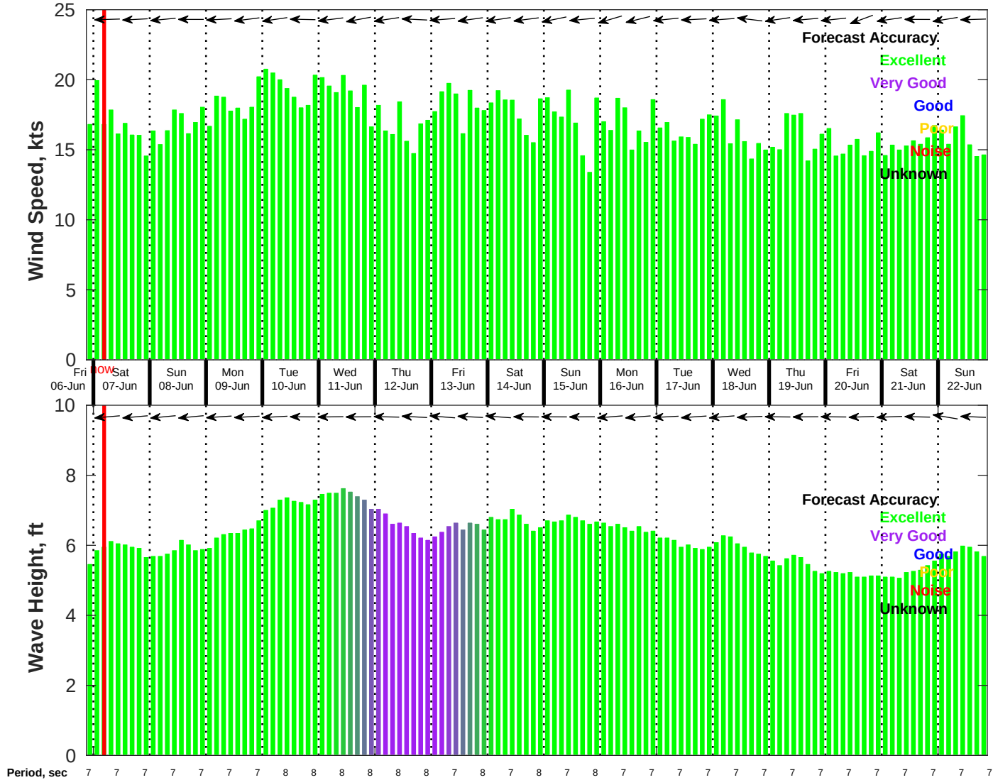
Wind & Wave Forecast for NDBC 41040 from 06-Jun-2025 21:00:00 to 22-Jun-2025 21:00:00
