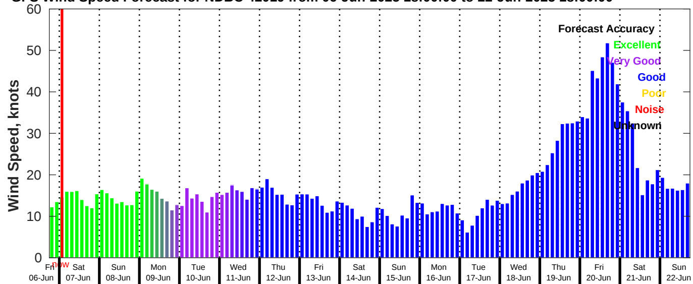
GFS Wind Speed Forecast for NDBC 42019 from 06-Jun-2025 18:00:00 to 22-Jun-2025 18:00:00
