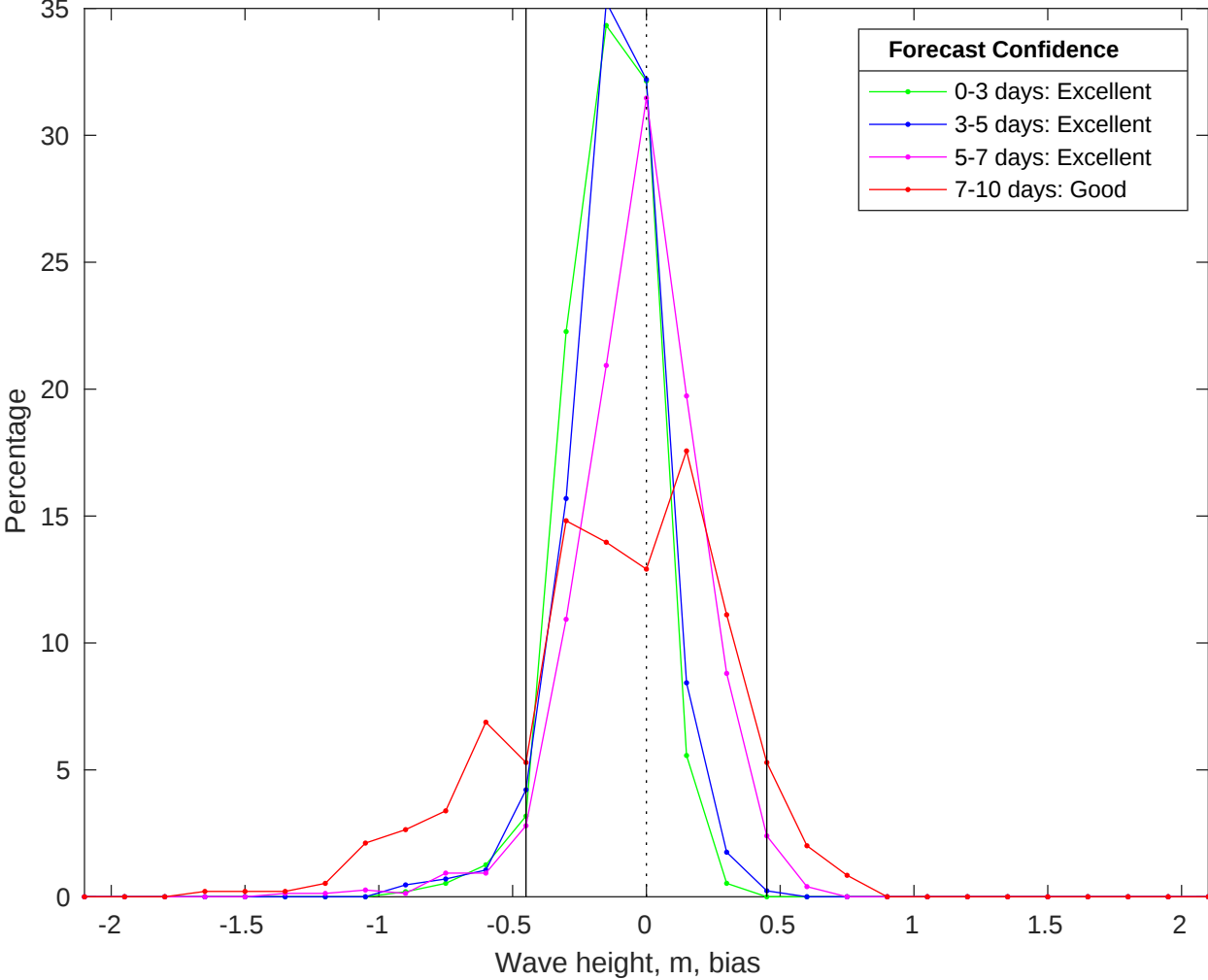
NDBC 42020 vs CMEMS Waves Bias Histogram: 07-Jun-2025
