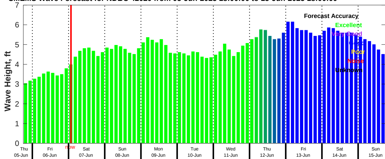
CMEMS Wave Forecast for NDBC 42020 from 05-Jun-2025 18:00:00 to 15-Jun-2025 18:00:00
