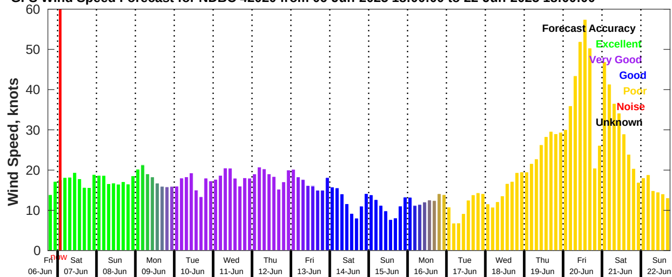
GFS Wind Speed Forecast for NDBC 42020 from 06-Jun-2025 18:00:00 to 22-Jun-2025 18:00:00
