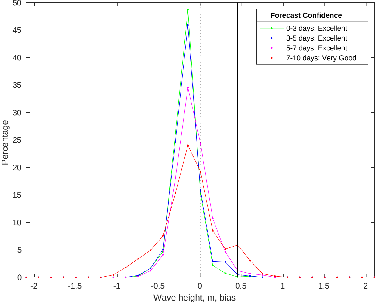
NDBC 42035 vs CMEMS Waves Bias Histogram: 07-Jun-2025
