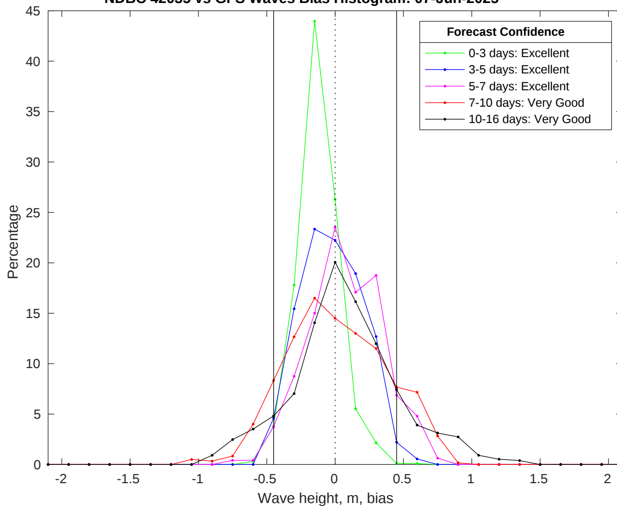
NDBC 42035 vs GFS Waves Bias Histogram: 07-Jun-2025
