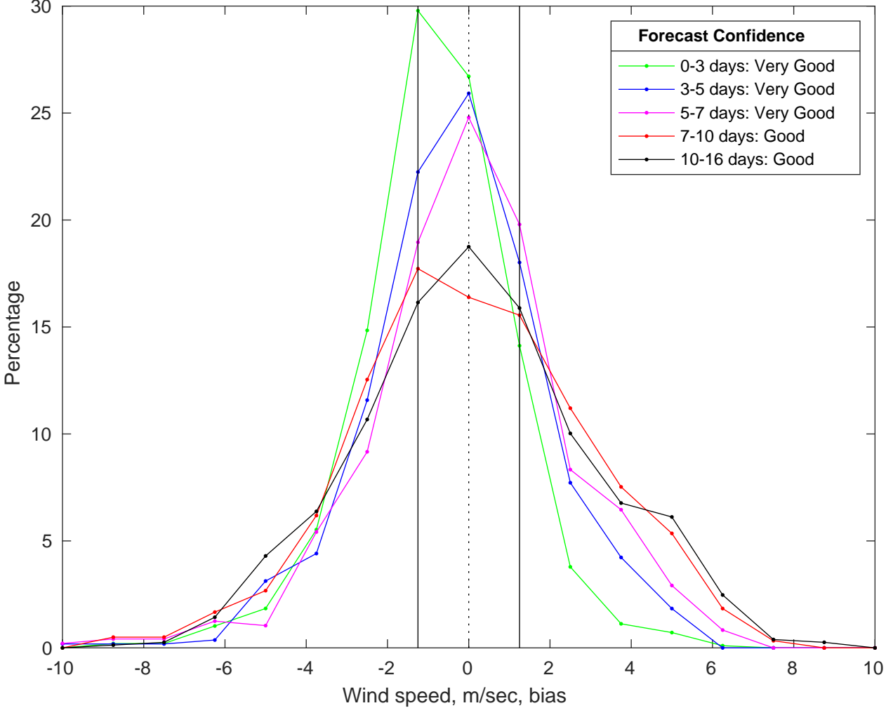
NDBC 42035 vs GFS Winds Bias Histogram: 07-Jun-2025
