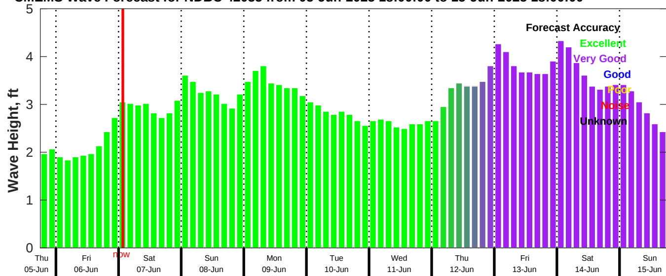
CMEMS Wave Forecast for NDBC 42035 from 05-Jun-2025 18:00:00 to 15-Jun-2025 18:00:00
