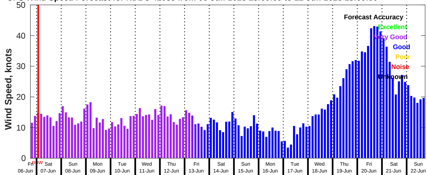
GFS Wind Speed Forecast for NDBC 42035 from 06-Jun-2025 18:00:00 to 22-Jun-2025 18:00:00
