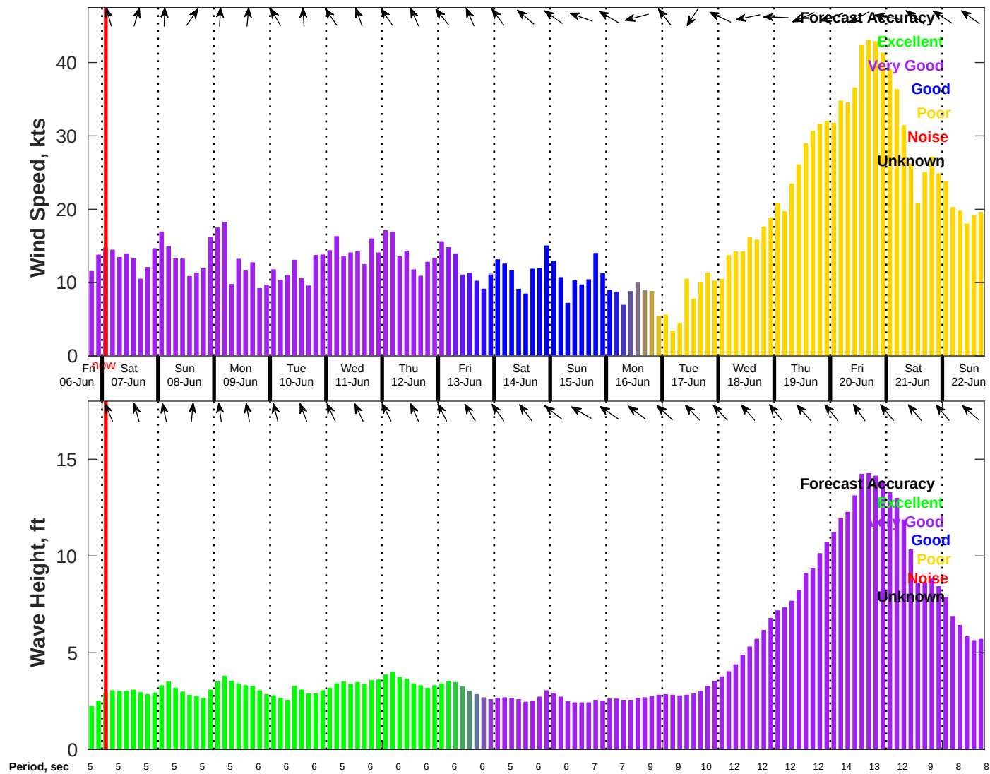
Wind & Wave Forecast for NDBC 42035 from 06-Jun-2025 18:00:00 to 22-Jun-2025 18:00:00
