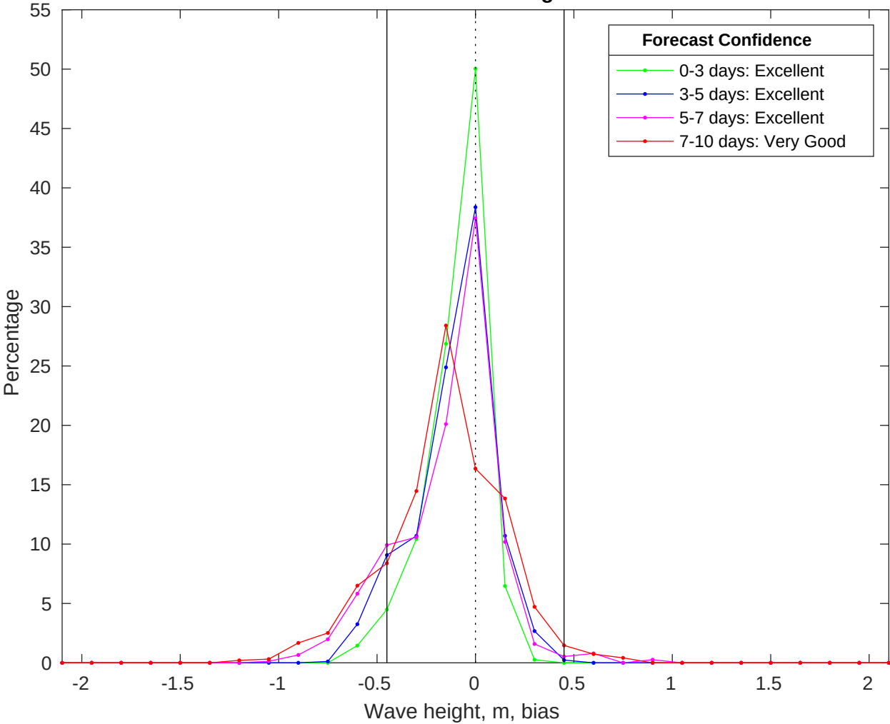
NDBC 42036 vs CMEMS Waves Bias Histogram: 07-Jun-2025
