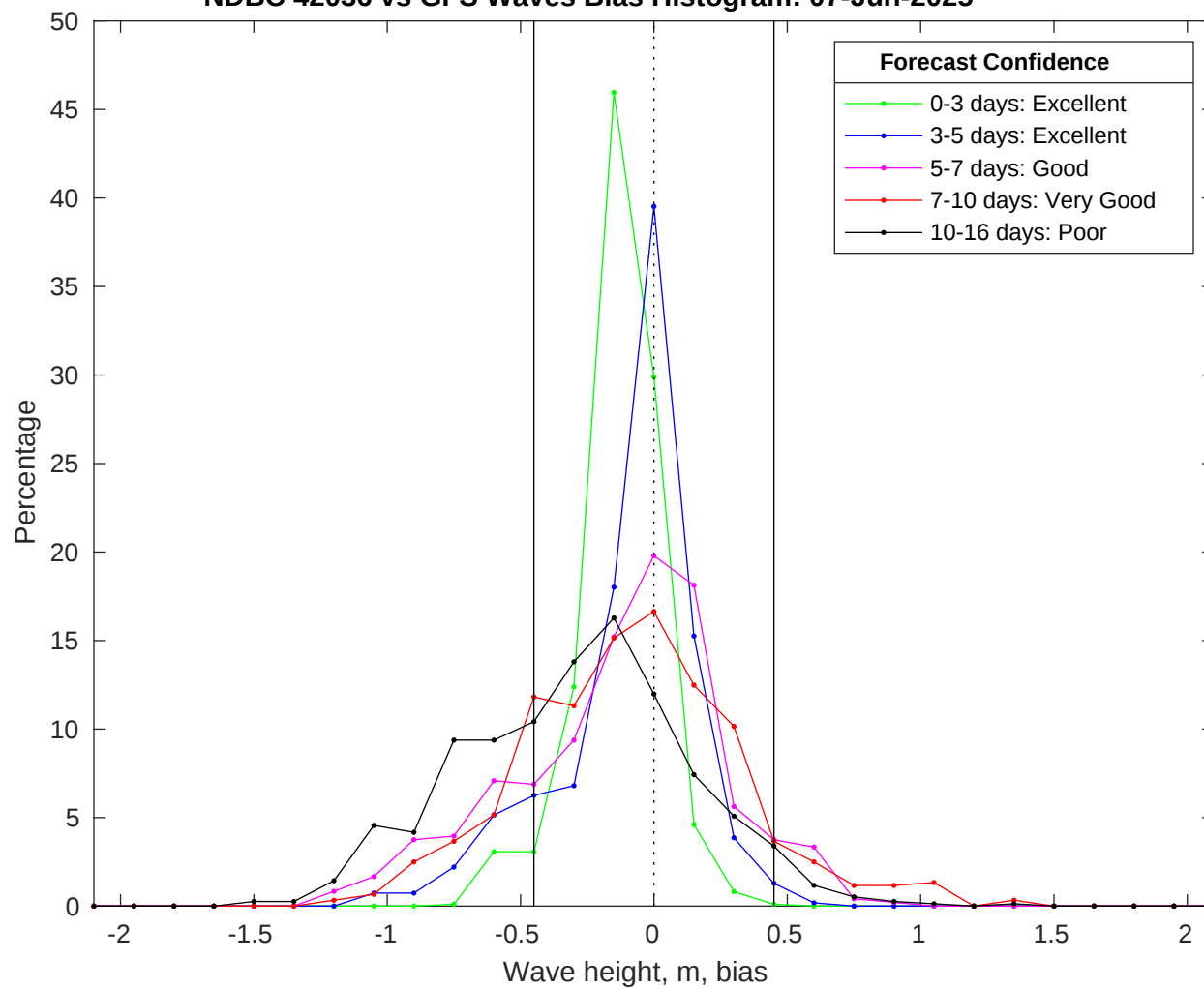
NDBC 42036 vs GFS Waves Bias Histogram: 07-Jun-2025
